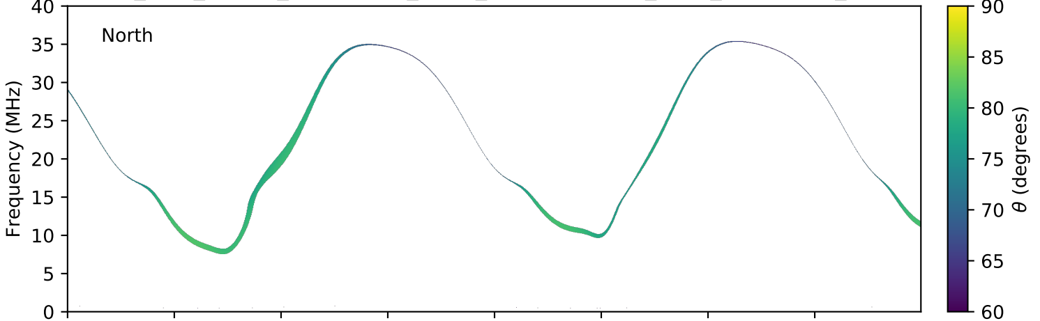
expres_juno_jupiter_ganymede_isaac_lossc-wid1deg_3kev_20171127_v01.cdf
