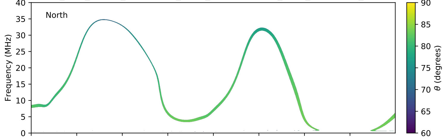
expres_juno_jupiter_ganymede_isaac_lossc-wid1deg_3kev_20171121_v01.cdf
