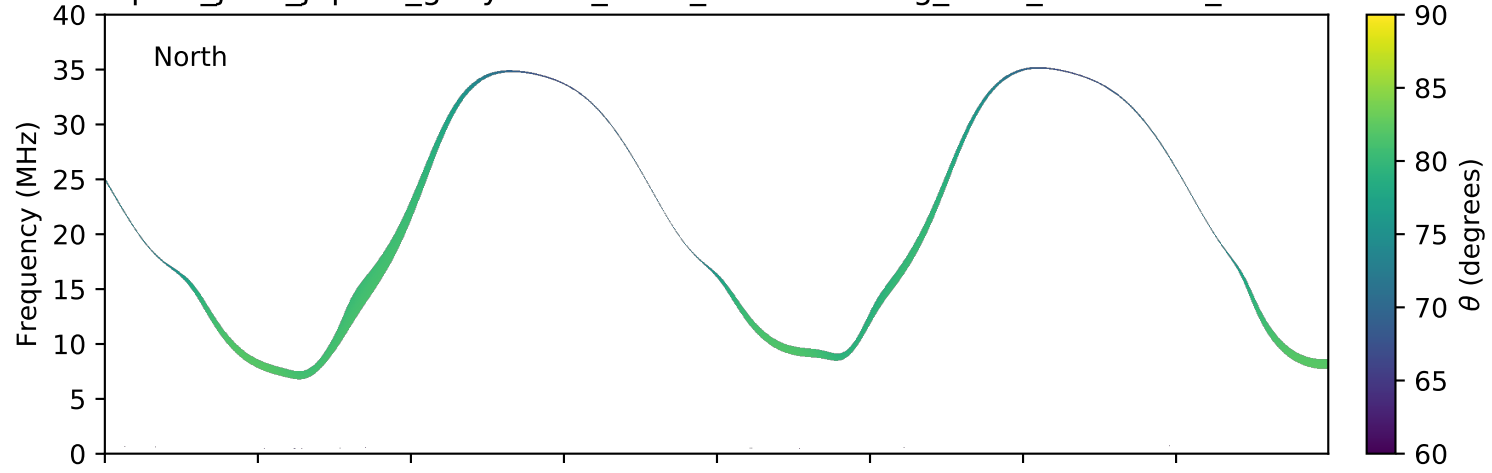
expres_juno_jupiter_ganymede_isaac_lossc-wid1deg_3kev_20171120_v01.cdf
