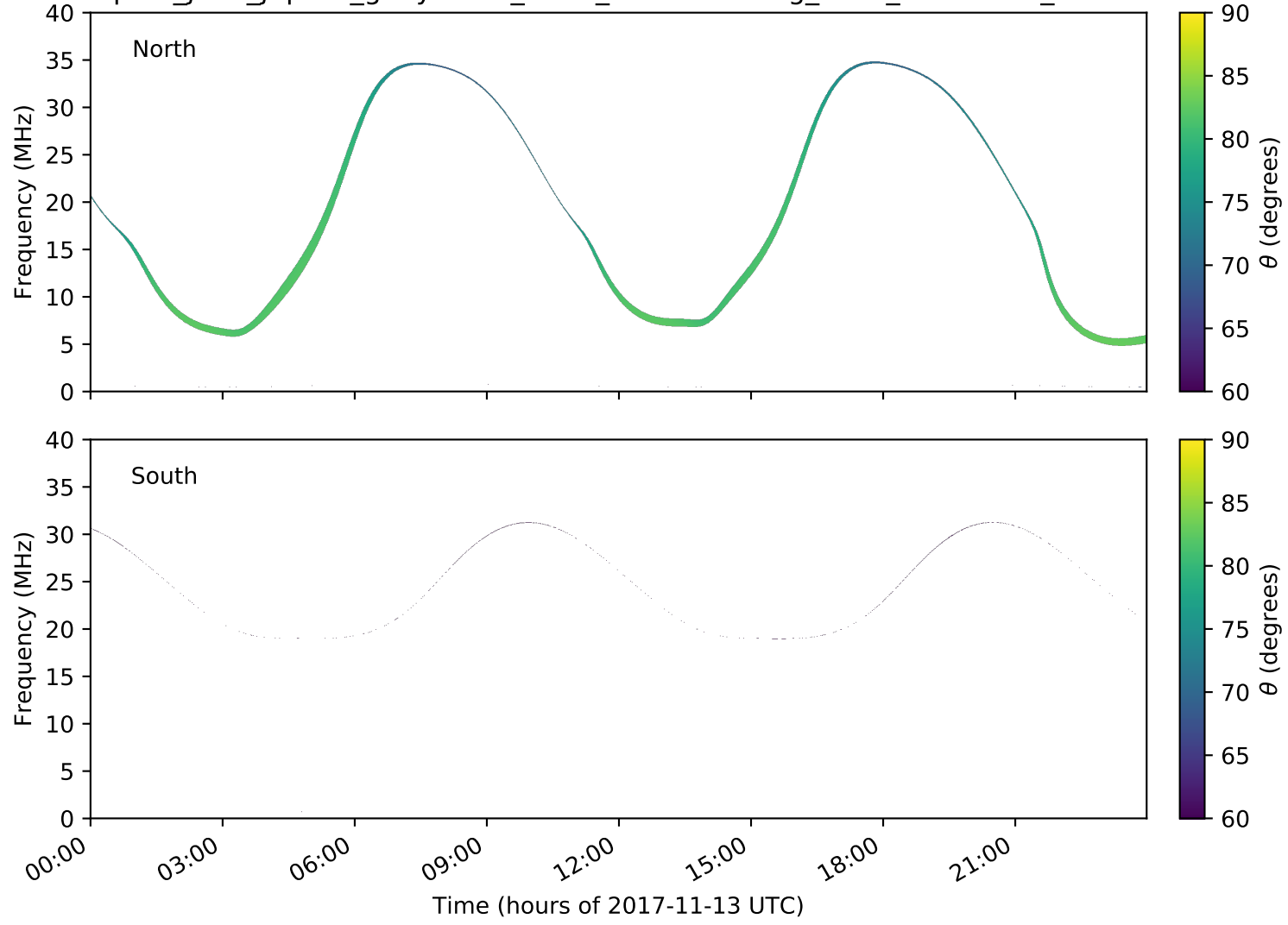
expres_juno_jupiter_ganymede_isaac_lossc-wid1deg_3kev_20171113_v01.cdf
