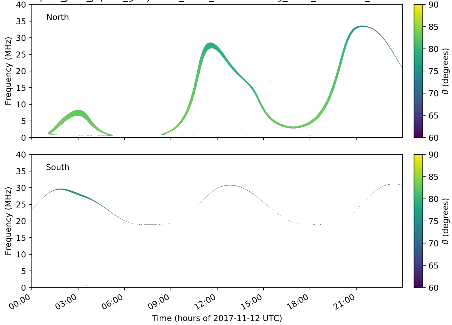
expres_juno_jupiter_ganymede_isaac_lossc-wid1deg_3kev_20171112_v01.cdf
