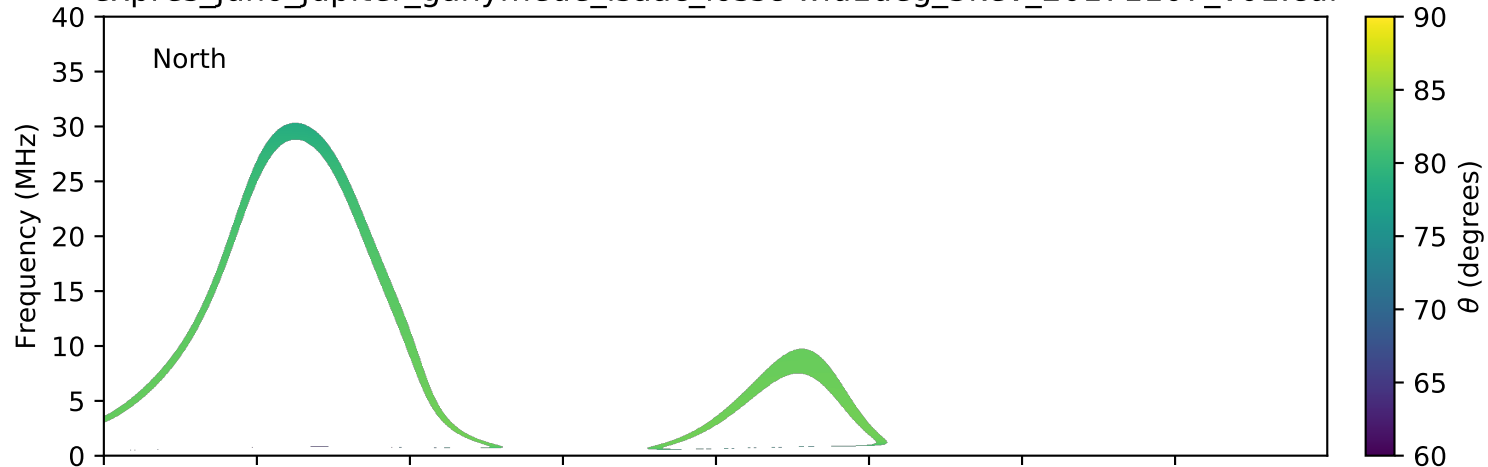
expres_juno_jupiter_ganymede_isaac_lossc-wid1deg_3kev_20171107_v01.cdf
