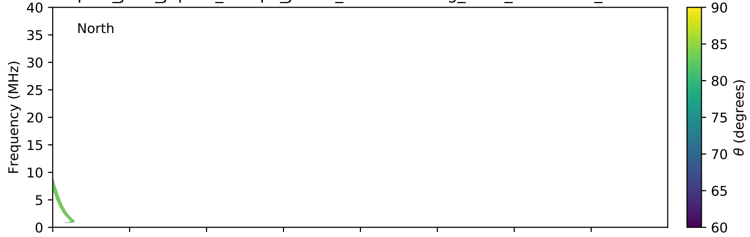
expres_juno_jupiter_europa_jrm09_lossc-wid1deg_3kev_20171130_v01.cdf
