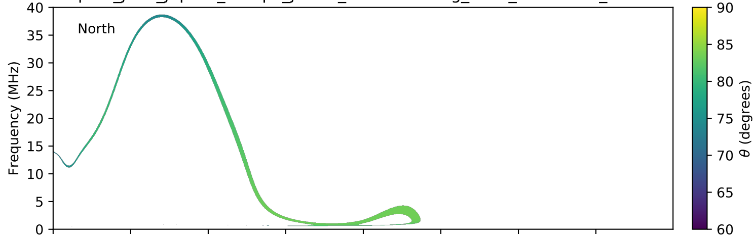
expres_juno_jupiter_europa_jrm09_lossc-wid1deg_3kev_20171126_v01.cdf
