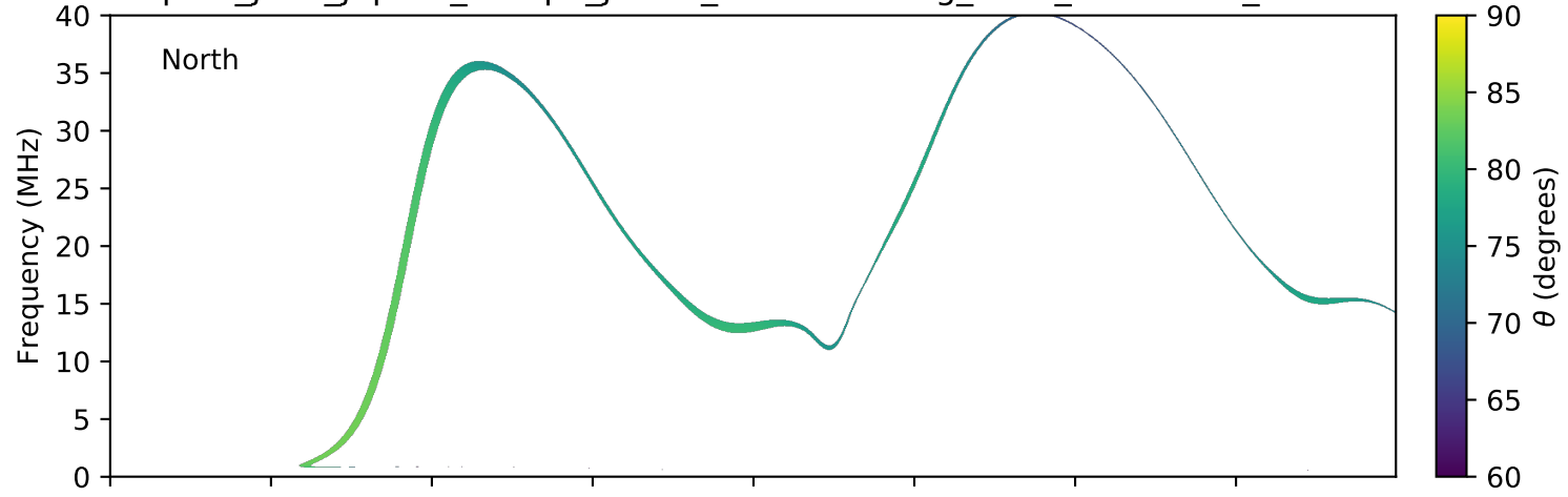
expres_juno_jupiter_europa_jrm09_lossc-wid1deg_3kev_20171125_v01.cdf
