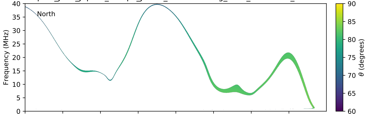
expres_juno_jupiter_europa_jrm09_lossc-wid1deg_3kev_20171122_v01.cdf
