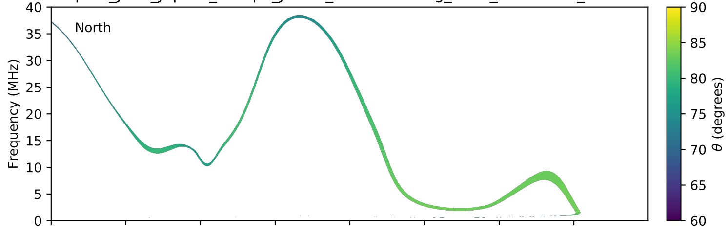
expres_juno_jupiter_europa_jrm09_lossc-wid1deg_3kev_20171115_v01.cdf
