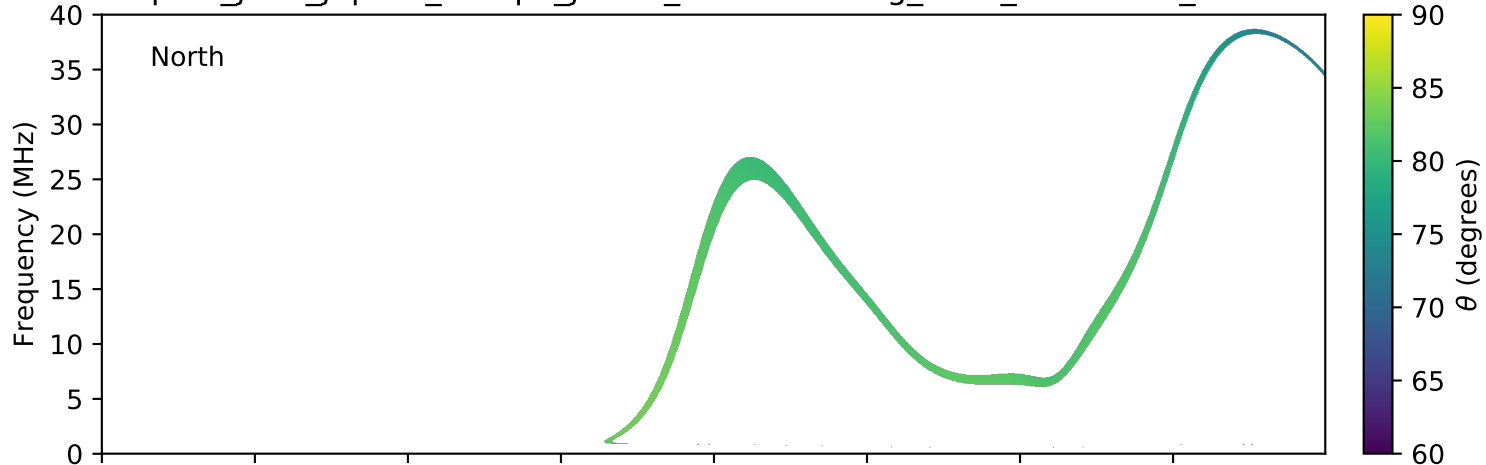
expres_juno_jupiter_europa_jrm09_lossc-wid1deg_3kev_20171107_v01.cdf
