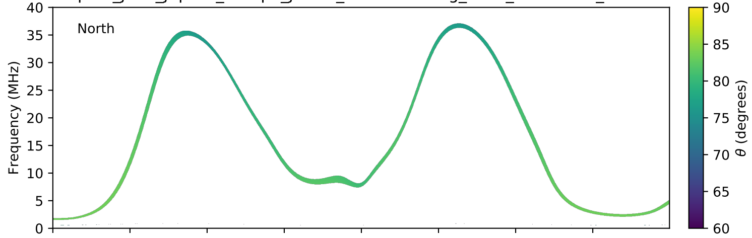
expres_juno_jupiter_europa_jrm09_lossc-wid1deg_3kev_20171104_v01.cdf
