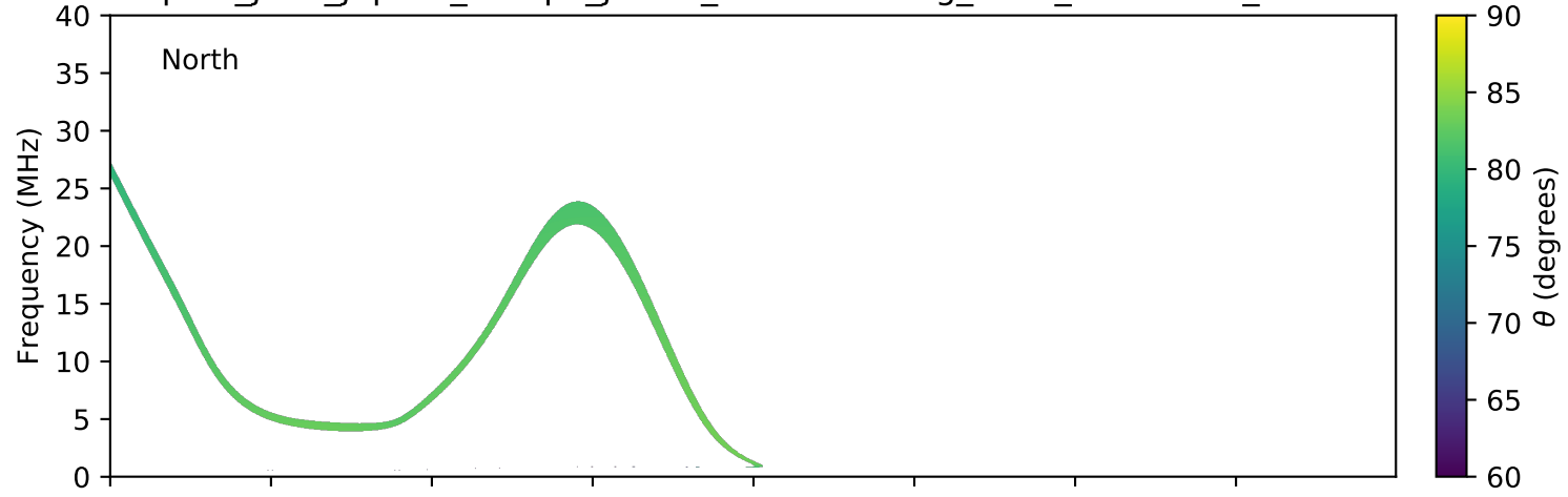
expres_juno_jupiter_europa_jrm09_lossc-wid1deg_3kev_20171101_v01.cdf
