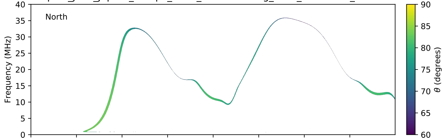
expres_juno_jupiter_europa_isaac_lossc-wid1deg_3kev_20171125_v01.cdf
