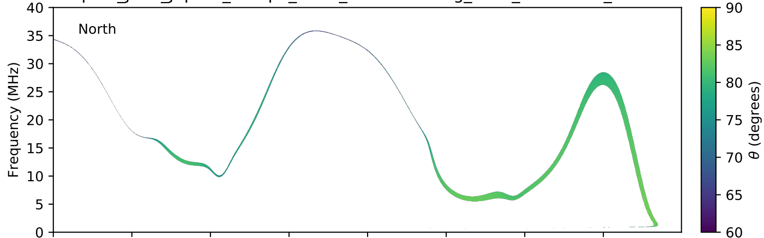
expres_juno_jupiter_europa_isaac_lossc-wid1deg_3kev_20171122_v01.cdf
