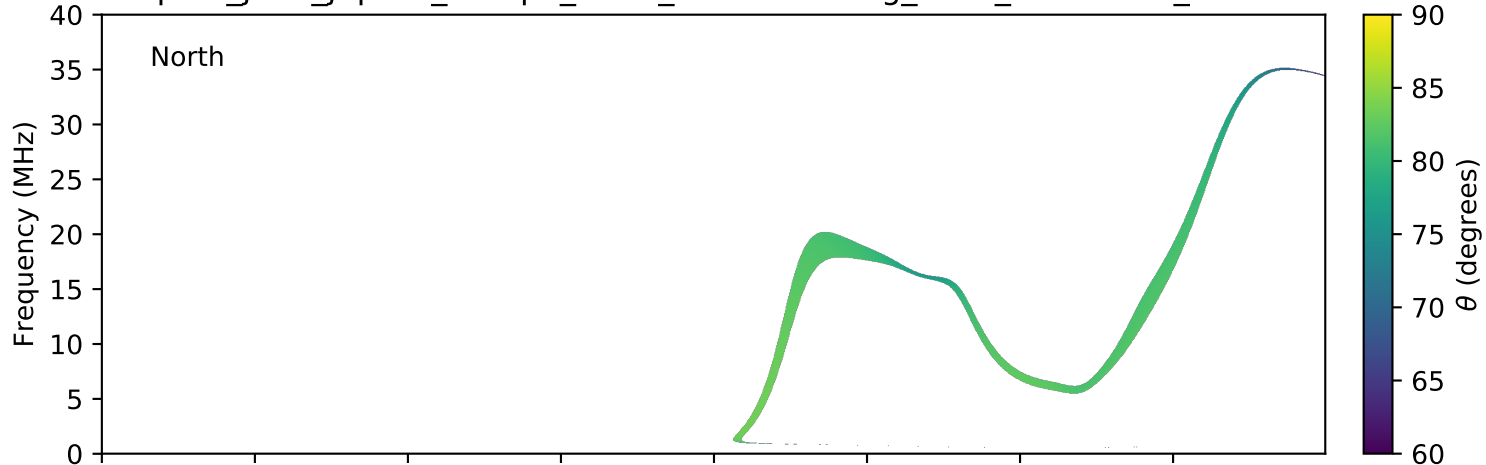
expres_juno_jupiter_europa_isaac_lossc-wid1deg_3kev_20171121_v01.cdf
