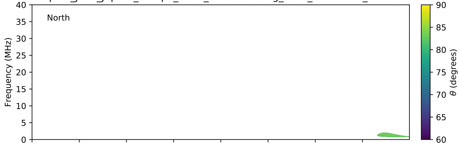
expres_juno_jupiter_europa_isaac_lossc-wid1deg_3kev_20171117_v01.cdf
