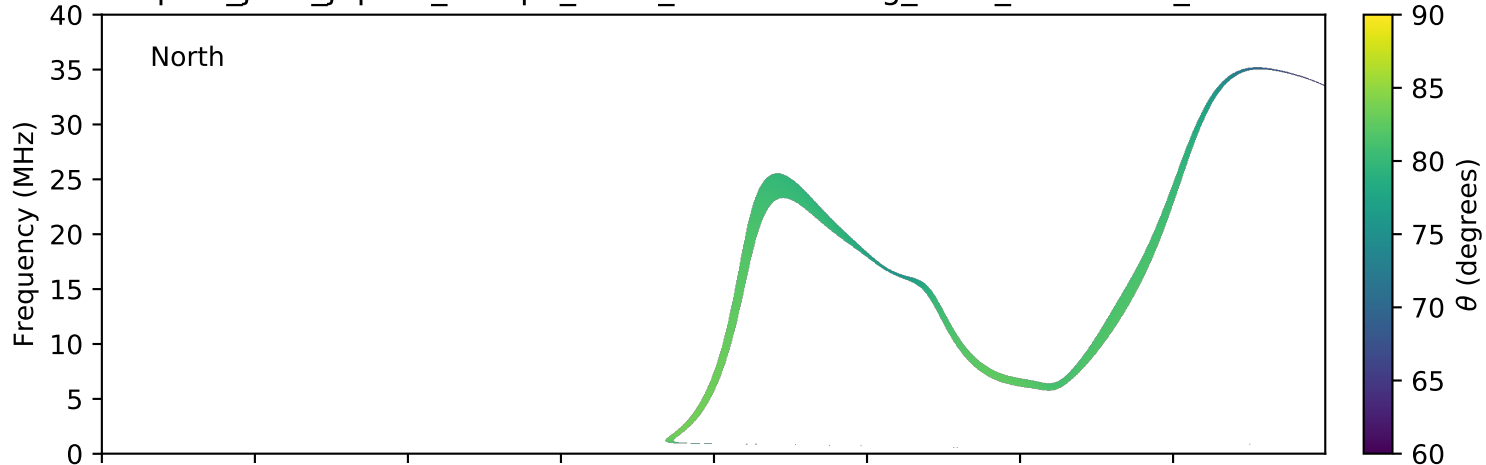
expres_juno_jupiter_europa_isaac_lossc-wid1deg_3kev_20171114_v01.cdf
