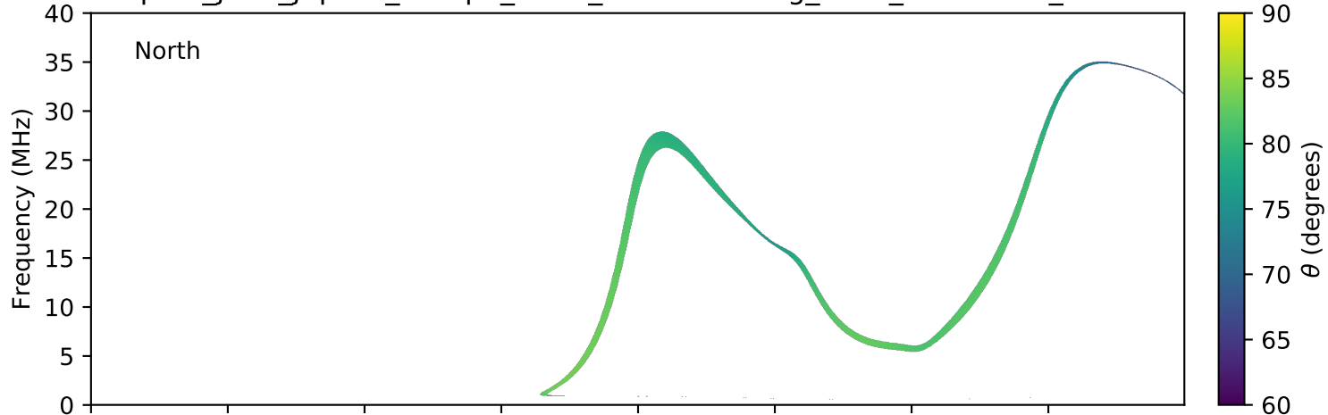
expres_juno_jupiter_europa_isaac_lossc-wid1deg_3kev_20171107_v01.cdf
