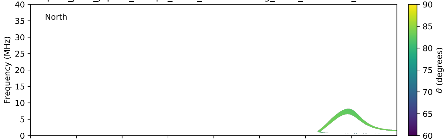
expres_juno_jupiter_europa_isaac_lossc-wid1deg_3kev_20171103_v01.cdf
