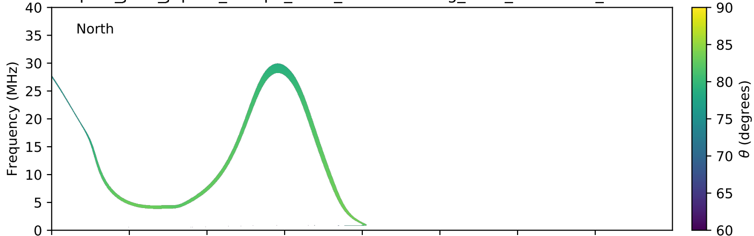
expres_juno_jupiter_europa_isaac_lossc-wid1deg_3kev_20171101_v01.cdf
