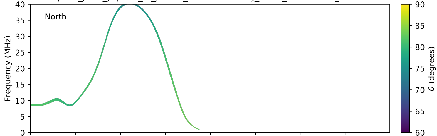
expres_juno_jupiter_io_jrm09_lossc-wid1deg_3kev_20171030_v01.cdf
