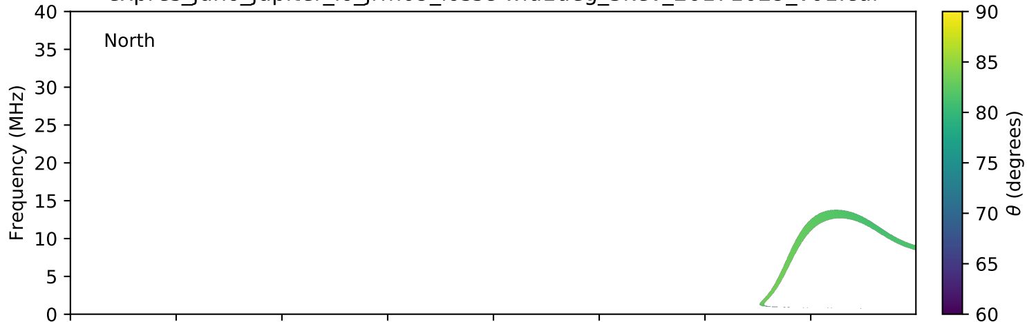
expres_juno_jupiter_io_jrm09_lossc-wid1deg_3kev_20171029_v01.cdf
