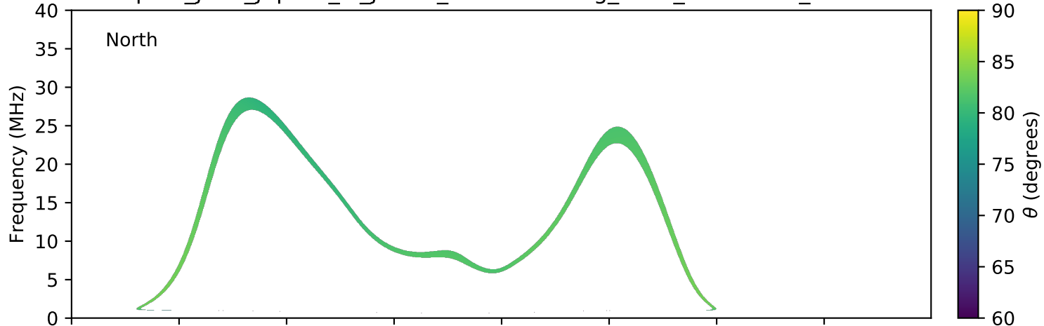
expres_juno_jupiter_io_jrm09_lossc-wid1deg_3kev_20171028_v01.cdf
