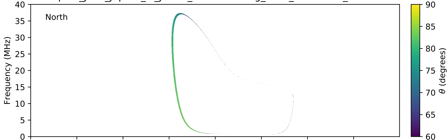
expres_juno_jupiter_io_jrm09_lossc-wid1deg_3kev_20171024_v01.cdf
