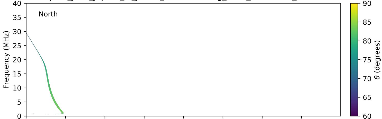
expres_juno_jupiter_io_jrm09_lossc-wid1deg_3kev_20171018_v01.cdf
