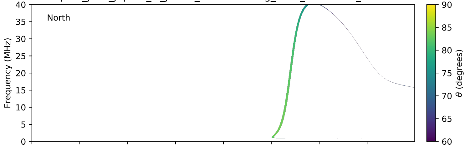
expres_juno_jupiter_io_jrm09_lossc-wid1deg_3kev_20171015_v01.cdf
