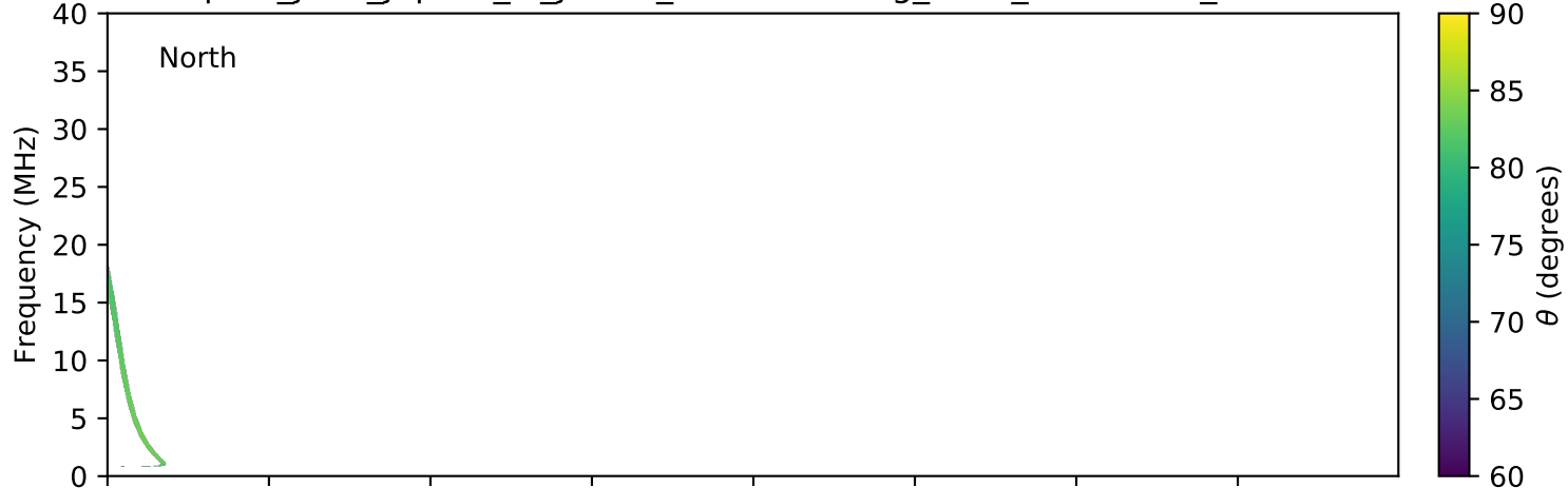
expres_juno_jupiter_io_jrm09_lossc-wid1deg_3kev_20171011_v01.cdf
