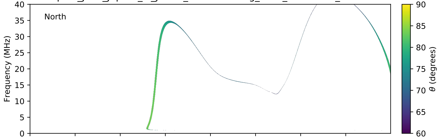
expres_juno_jupiter_io_jrm09_lossc-wid1deg_3kev_20171010_v01.cdf
