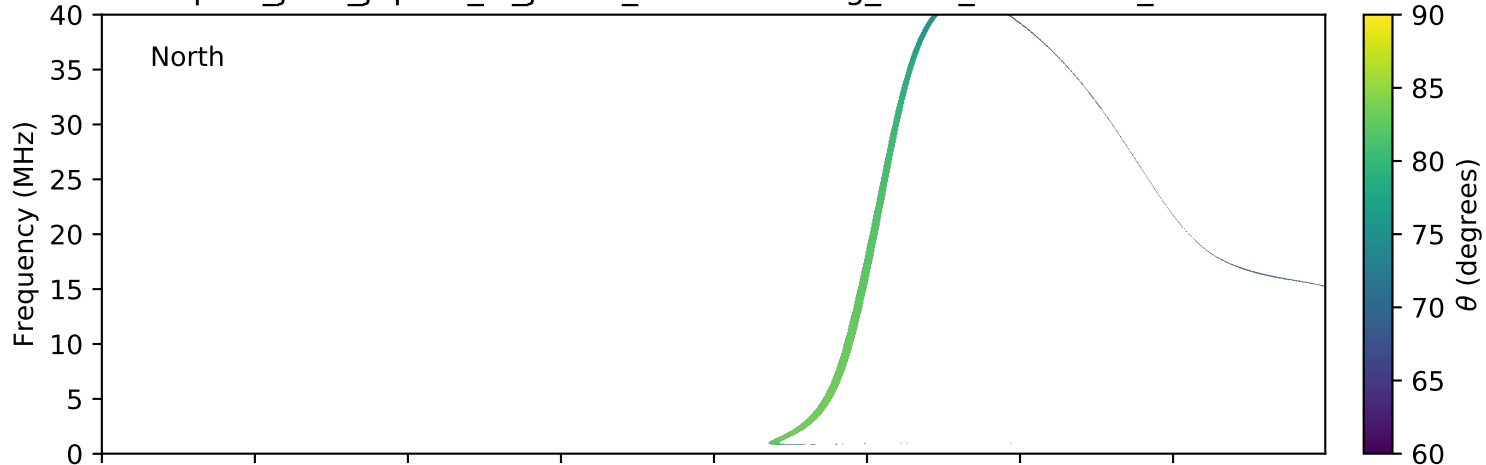
expres_juno_jupiter_io_jrm09_lossc-wid1deg_3kev_20171008_v01.cdf
