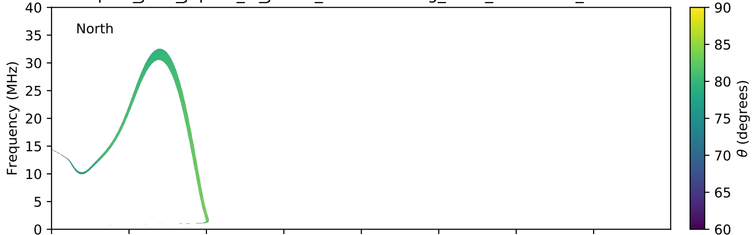
expres_juno_jupiter_io_jrm09_lossc-wid1deg_3kev_20171002_v01.cdf
