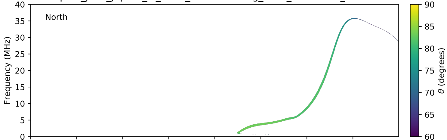
expres_juno_jupiter_io_isaac_lossc-wid1deg_3kev_20171031_v01.cdf
