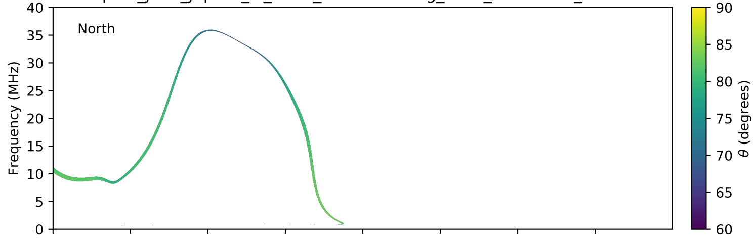
expres_juno_jupiter_io_isaac_lossc-wid1deg_3kev_20171030_v01.cdf
