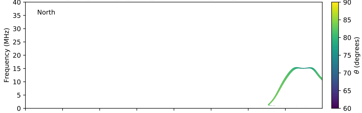
expres_juno_jupiter_io_isaac_lossc-wid1deg_3kev_20171029_v01.cdf
