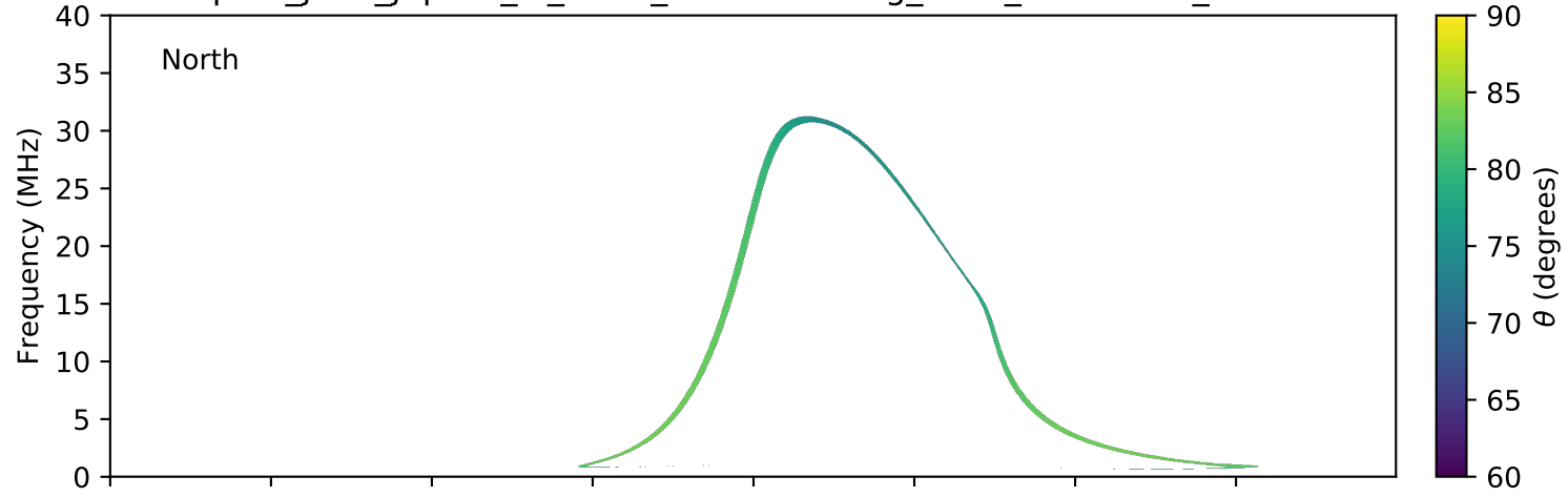
expres_juno_jupiter_io_isaac_lossc-wid1deg_3kev_20171026_v01.cdf
