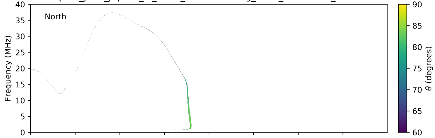
expres_juno_jupiter_io_isaac_lossc-wid1deg_3kev_20171023_v01.cdf
