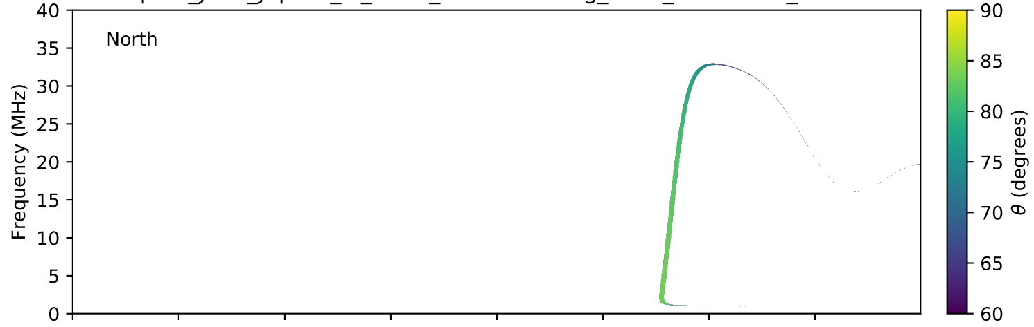
expres_juno_jupiter_io_isaac_lossc-wid1deg_3kev_20171022_v01.cdf
