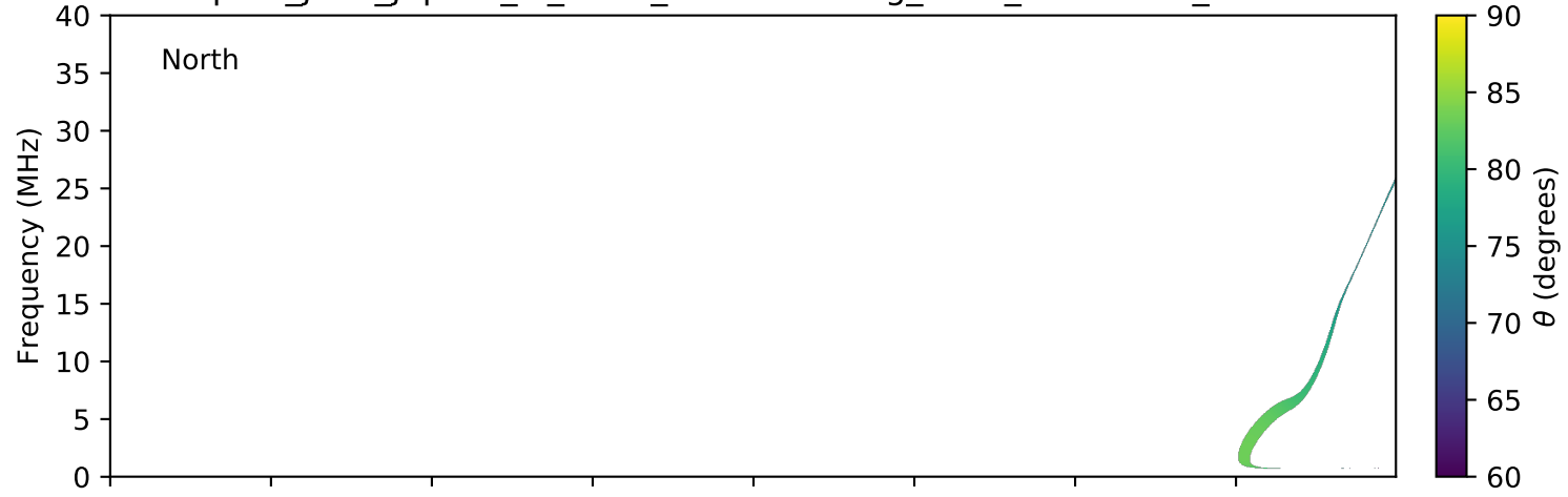
expres_juno_jupiter_io_isaac_lossc-wid1deg_3kev_20171020_v01.cdf
