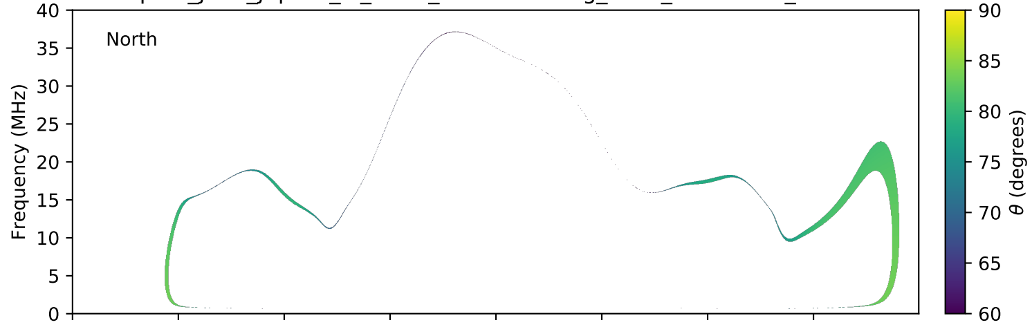
expres_juno_jupiter_io_isaac_lossc-wid1deg_3kev_20171019_v01.cdf
