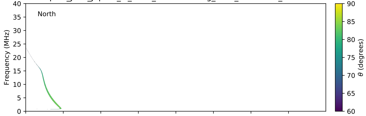
expres_juno_jupiter_io_isaac_lossc-wid1deg_3kev_20171018_v01.cdf
