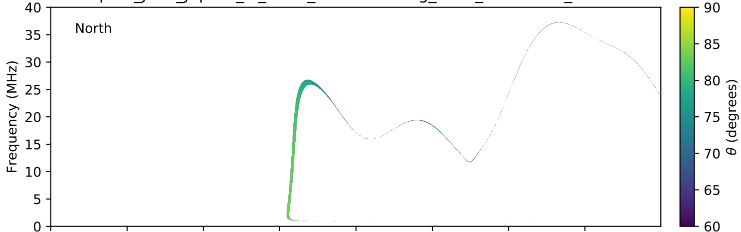
expres_juno_jupiter_io_isaac_lossc-wid1deg_3kev_20171017_v01.cdf
