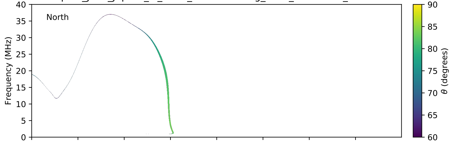
expres_juno_jupiter_io_isaac_lossc-wid1deg_3kev_20171016_v01.cdf
