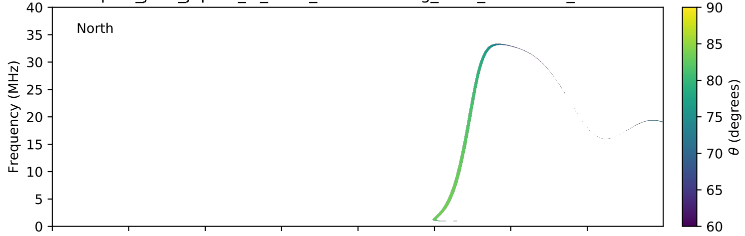
expres_juno_jupiter_io_isaac_lossc-wid1deg_3kev_20171015_v01.cdf
