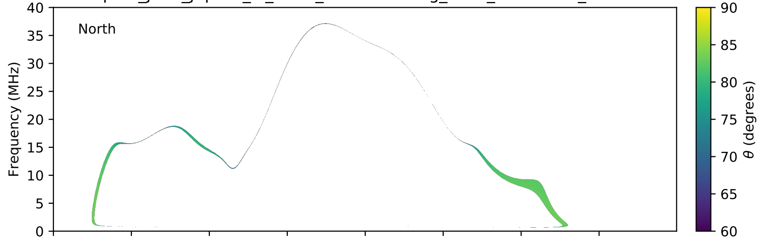
expres_juno_jupiter_io_isaac_lossc-wid1deg_3kev_20171012_v01.cdf
