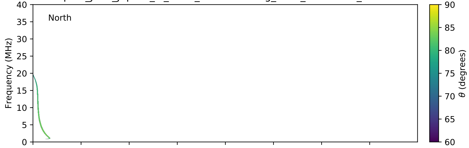
expres_juno_jupiter_io_isaac_lossc-wid1deg_3kev_20171011_v01.cdf
