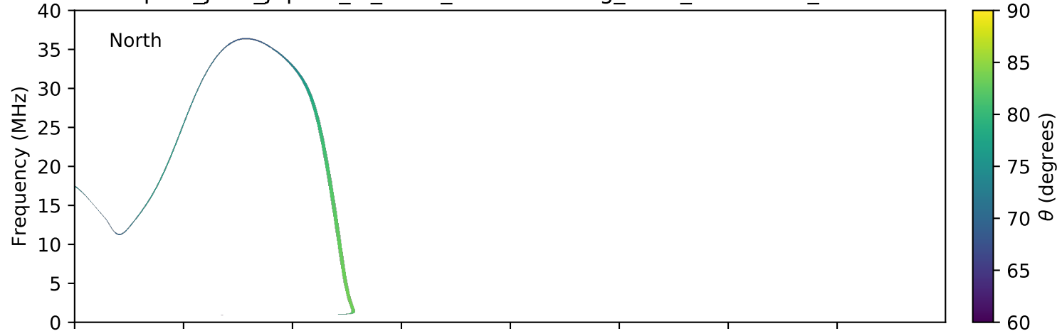
expres_juno_jupiter_io_isaac_lossc-wid1deg_3kev_20171009_v01.cdf
