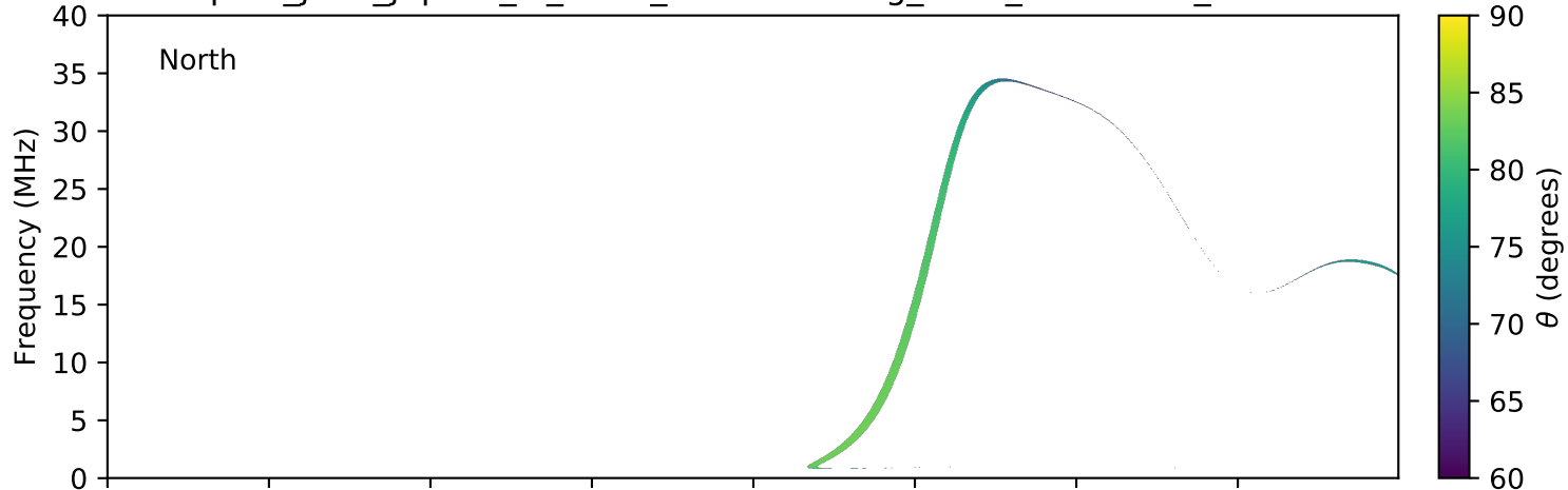
expres_juno_jupiter_io_isaac_lossc-wid1deg_3kev_20171008_v01.cdf
