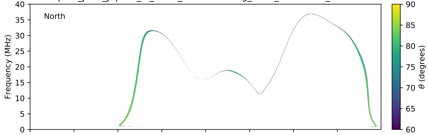
expres_juno_jupiter_io_isaac_lossc-wid1deg_3kev_20171003_v01.cdf
