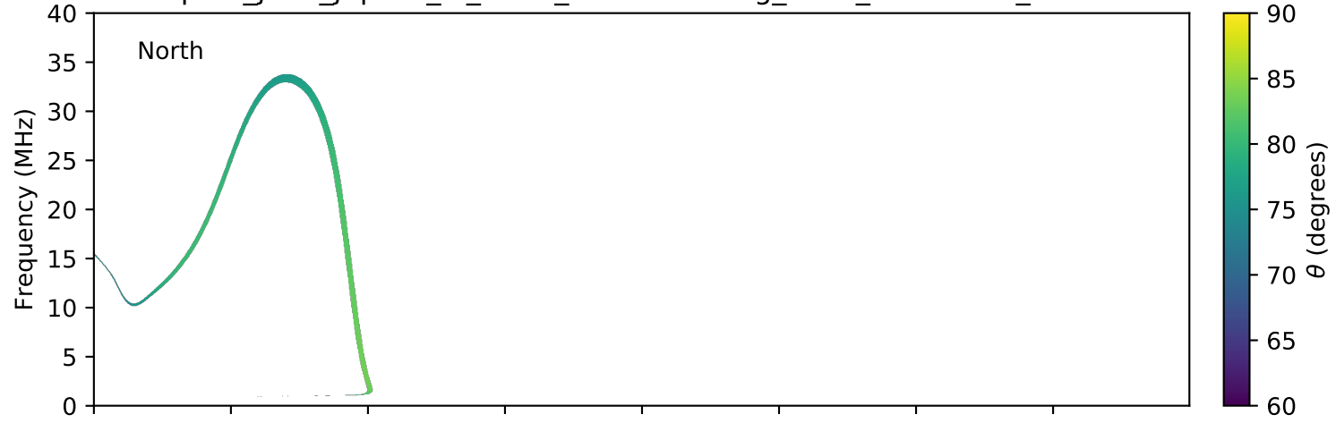
expres_juno_jupiter_io_isaac_lossc-wid1deg_3kev_20171002_v01.cdf
